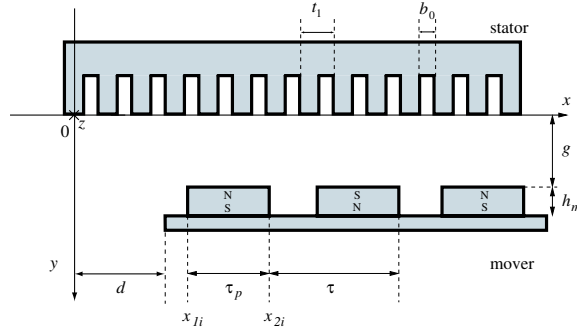
Figure 2: Inertial frame of a single PMLSM
