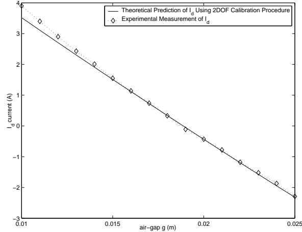
Figure 9: Comparing predicted i_d current with actual measurement
