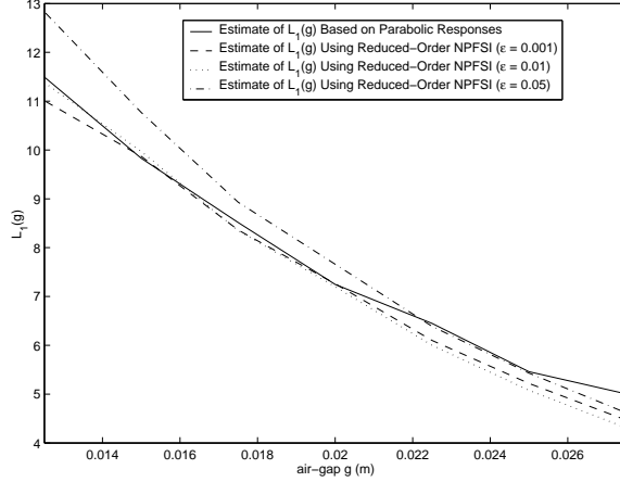
Figure 4: Comparison of various estimations of L_1(x_1)
