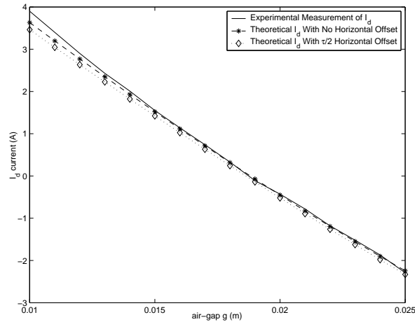
Figure 7: Measured and theoretical equilibrium i_d currents at each air-gap
