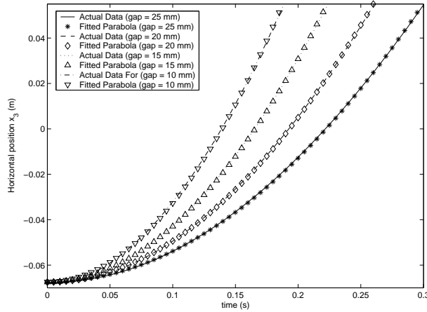
Figure 3: Some results of parabolic curve-fitting to position data
