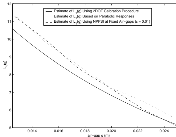
Figure 8: Comparison between various estimates of L_1(g)
