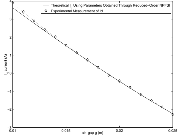
Figure 5: Comparing measured i_d currents and the theoretical predictions
