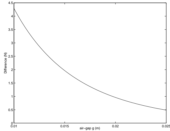
Figure 6: Estimate of the peak cogging force over the entire air-gap range
