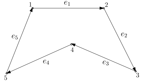
(c) non-collinear: |e_i| = b, \forall i .
